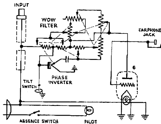
Schematic Diagram
