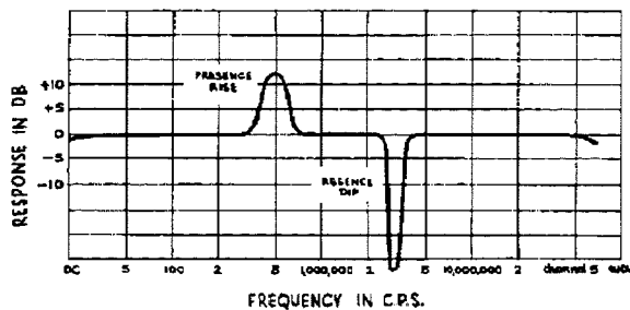
Fig. 3 - Frequency Response at 791-watt Level
