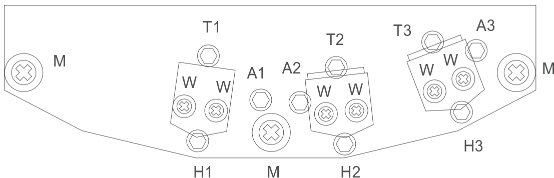
Figure 6-9 Head Assembly
