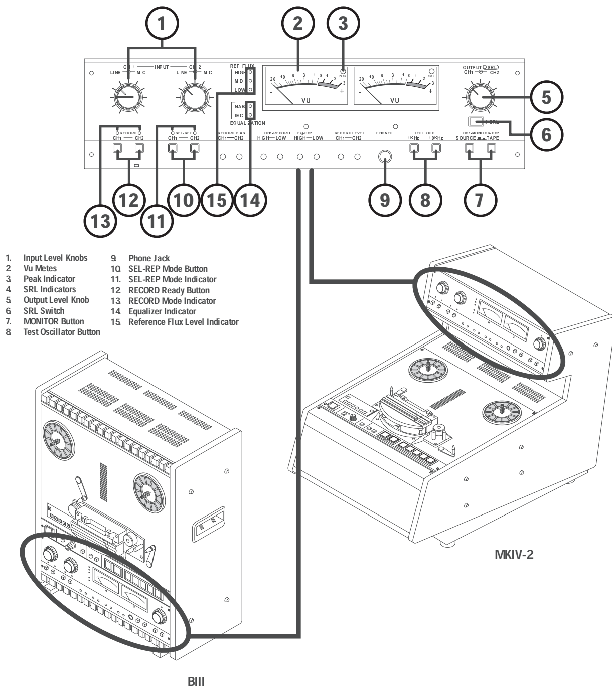
Figure 3-4 Amplifier Panel
