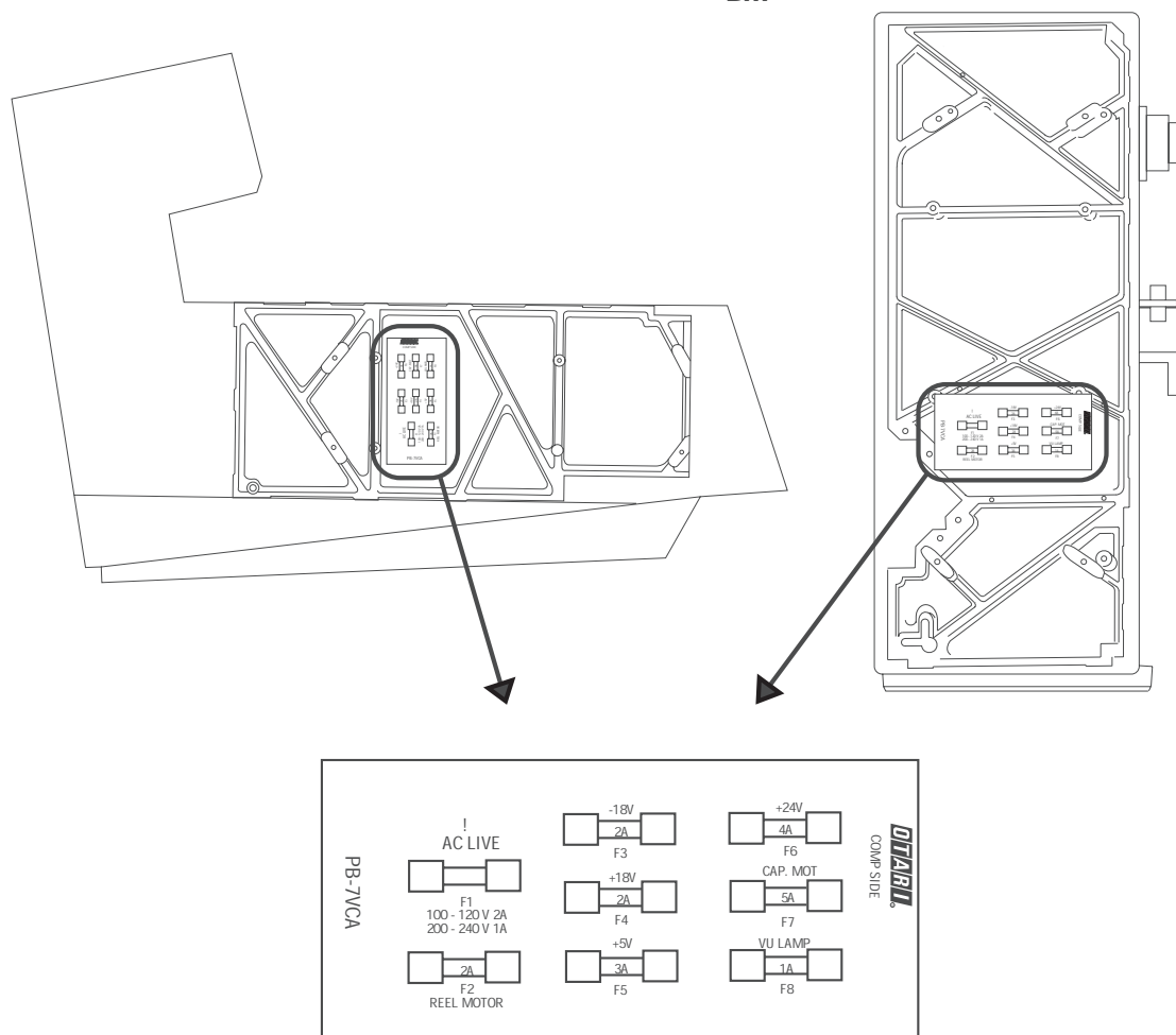
Figure 2-12 Fuse Location
