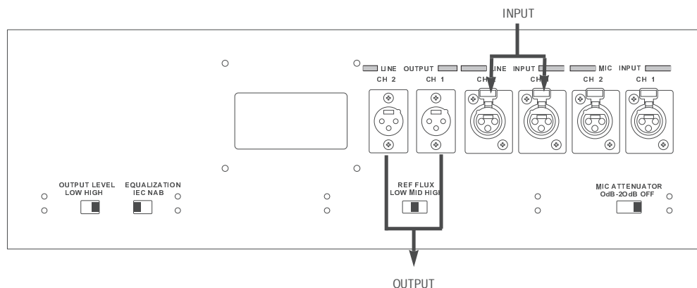
Figure 2-1 Input/Output Connectors
