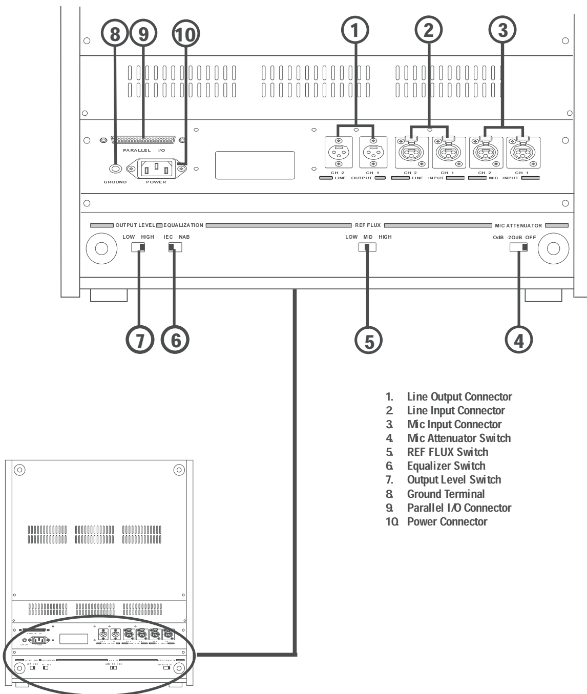
Figure 3-5 Audio Connector Panel (BIII)
