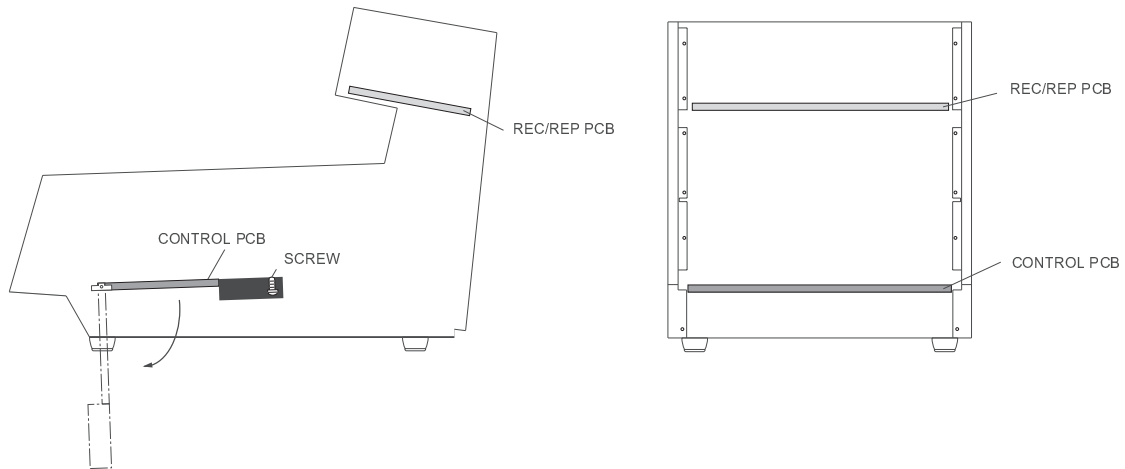
Figure 2-8 PCB Assembly Location
