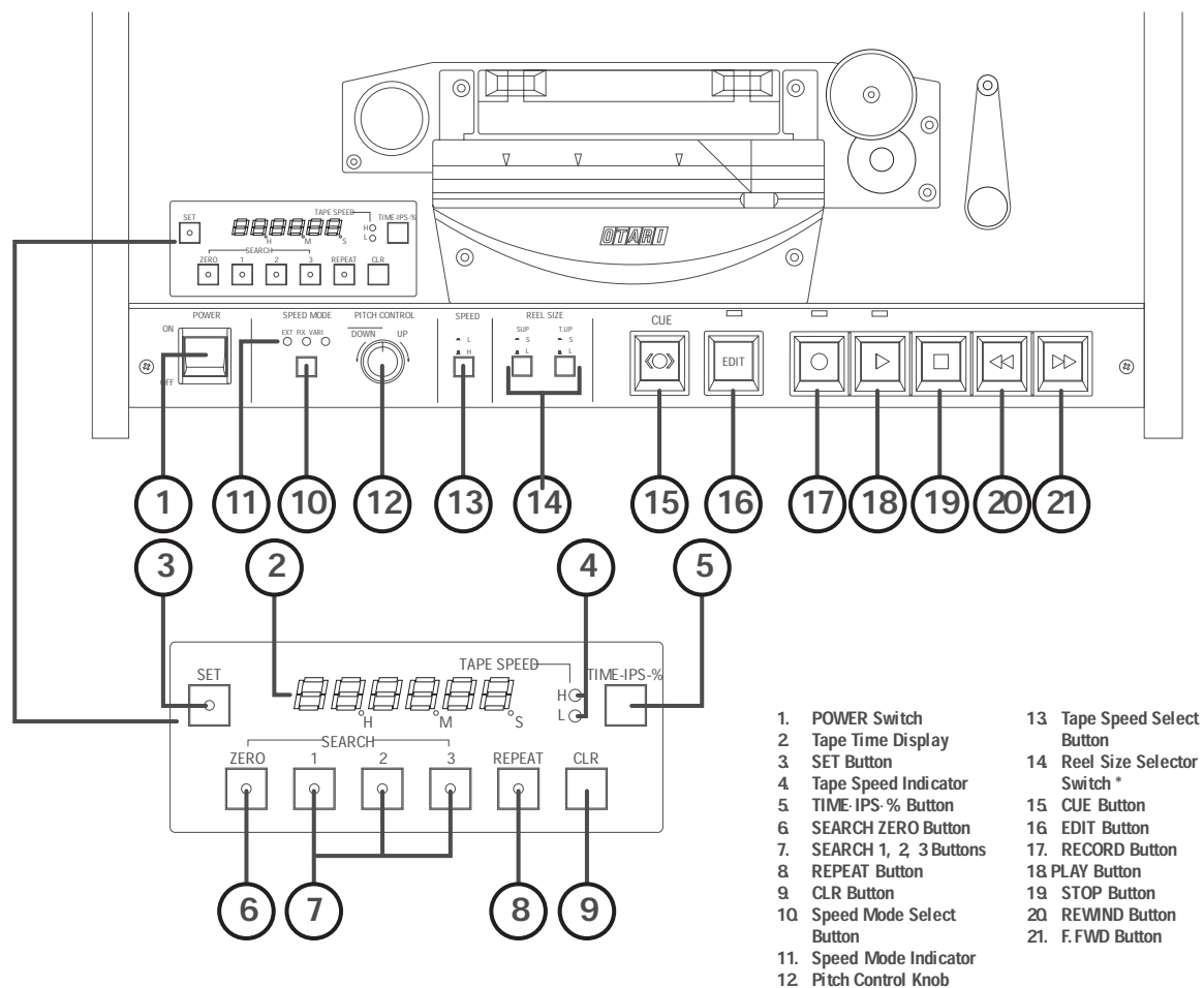
Figure 3-2 Transport Control Panel
